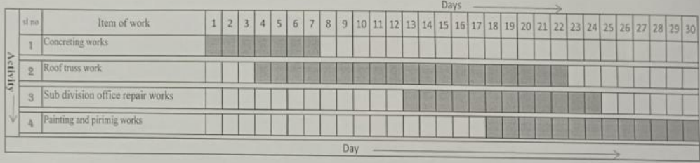
Bar Chart for the work, "Protection of roof by steel truss for office of the Sub-Divisional Officer of Karatowa Talma Barrage Sub-Division under Mahananda Link Canal Division at Ambari Falakata, in P.S- Rajganj, Dist.- Jalpaiguri."
