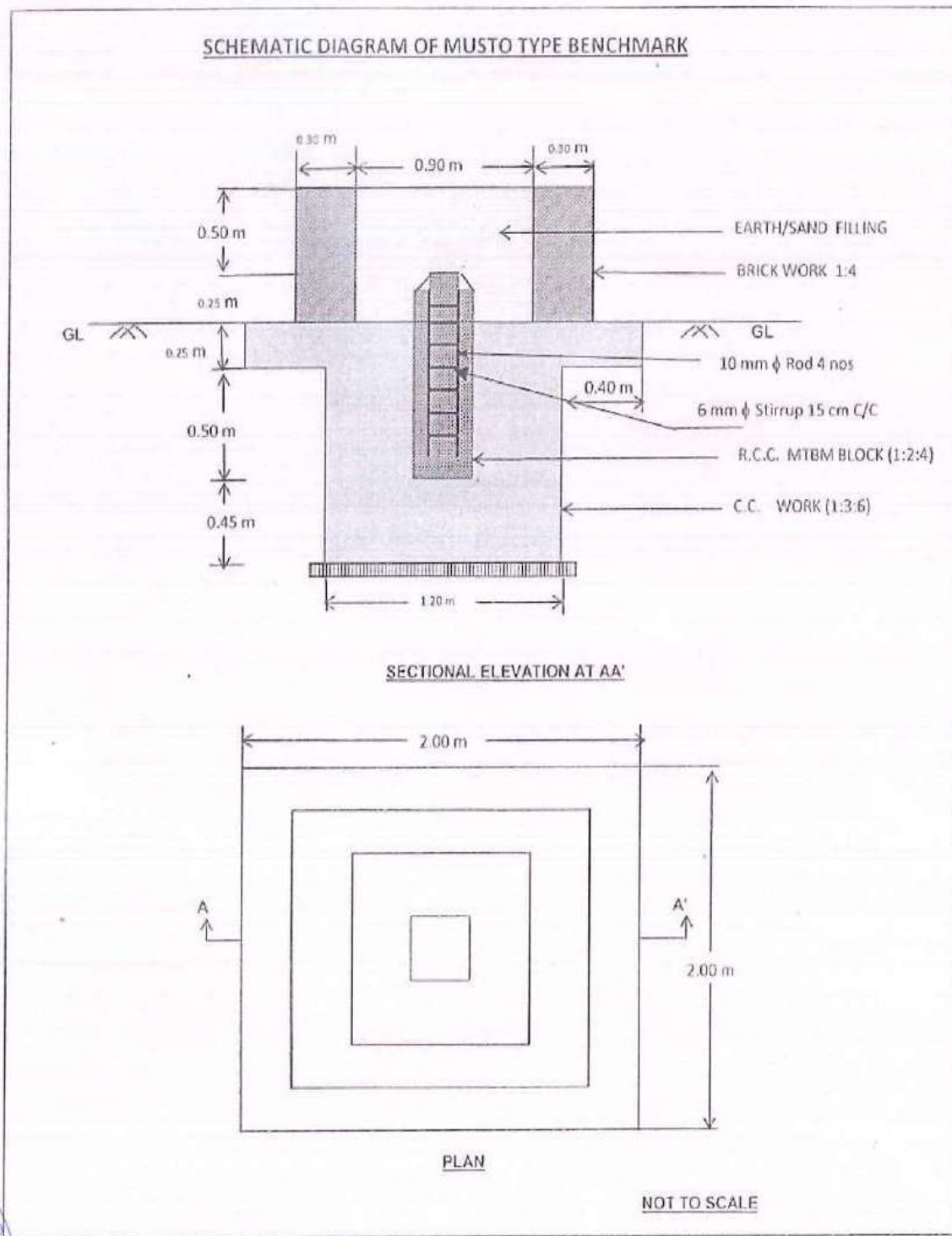
TYPICAL SECTION OF BM PILLAR
