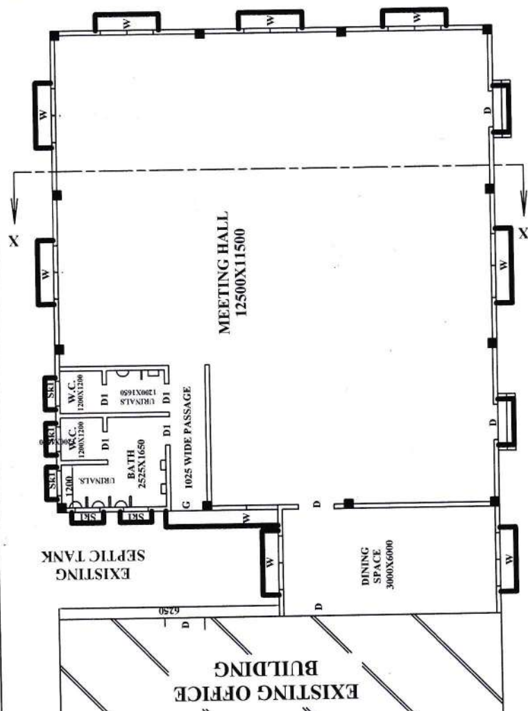
PLAN OF MEETING HALL WITHIN POSHPUR OFFICE COMPOUND
