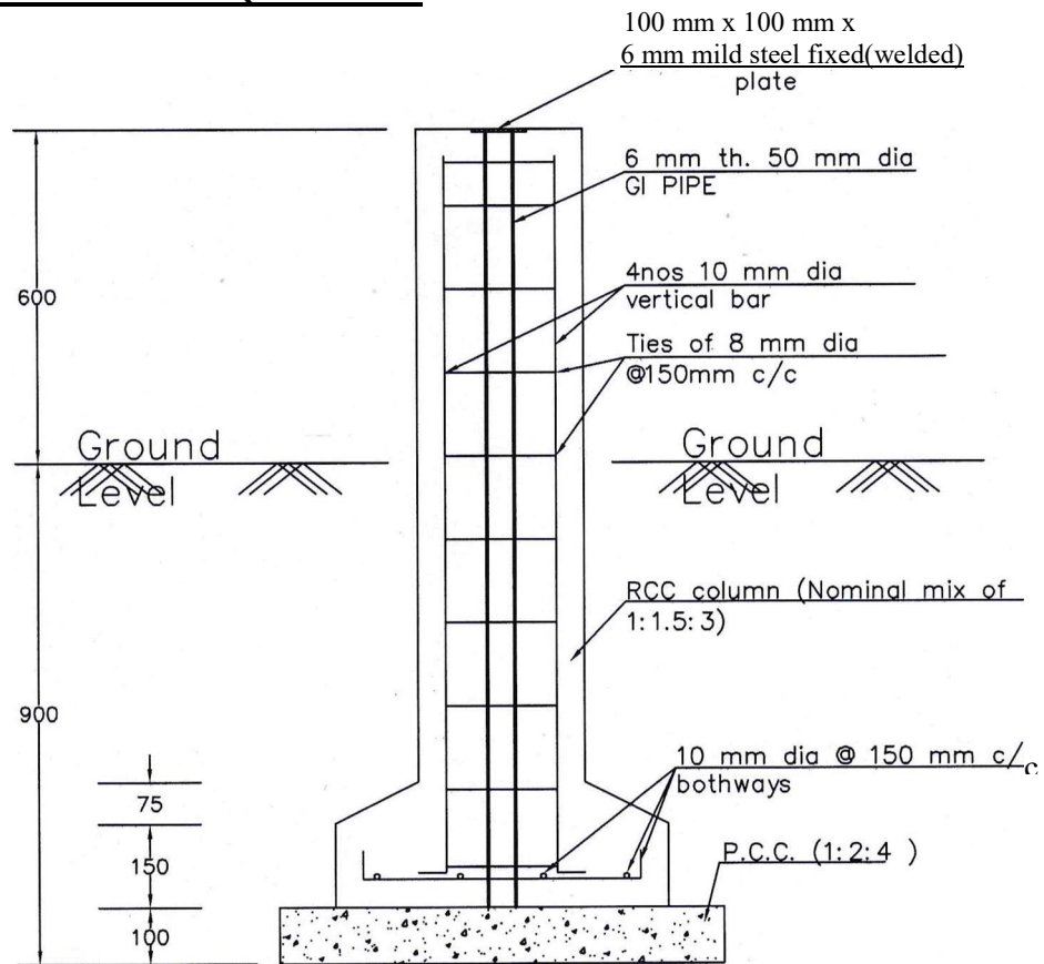
SECTIONAL ELEVATION
