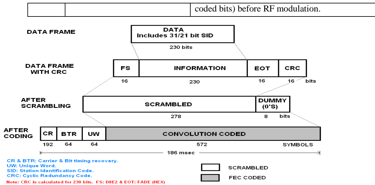
Fig. 1: Burst Transmission Format for TDMA Technique (4800 Symbols/sec.)
