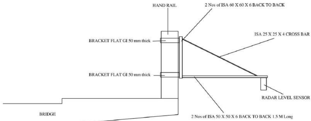
RADAR SENSOR FARMING TO BRIDGE DETAILS
